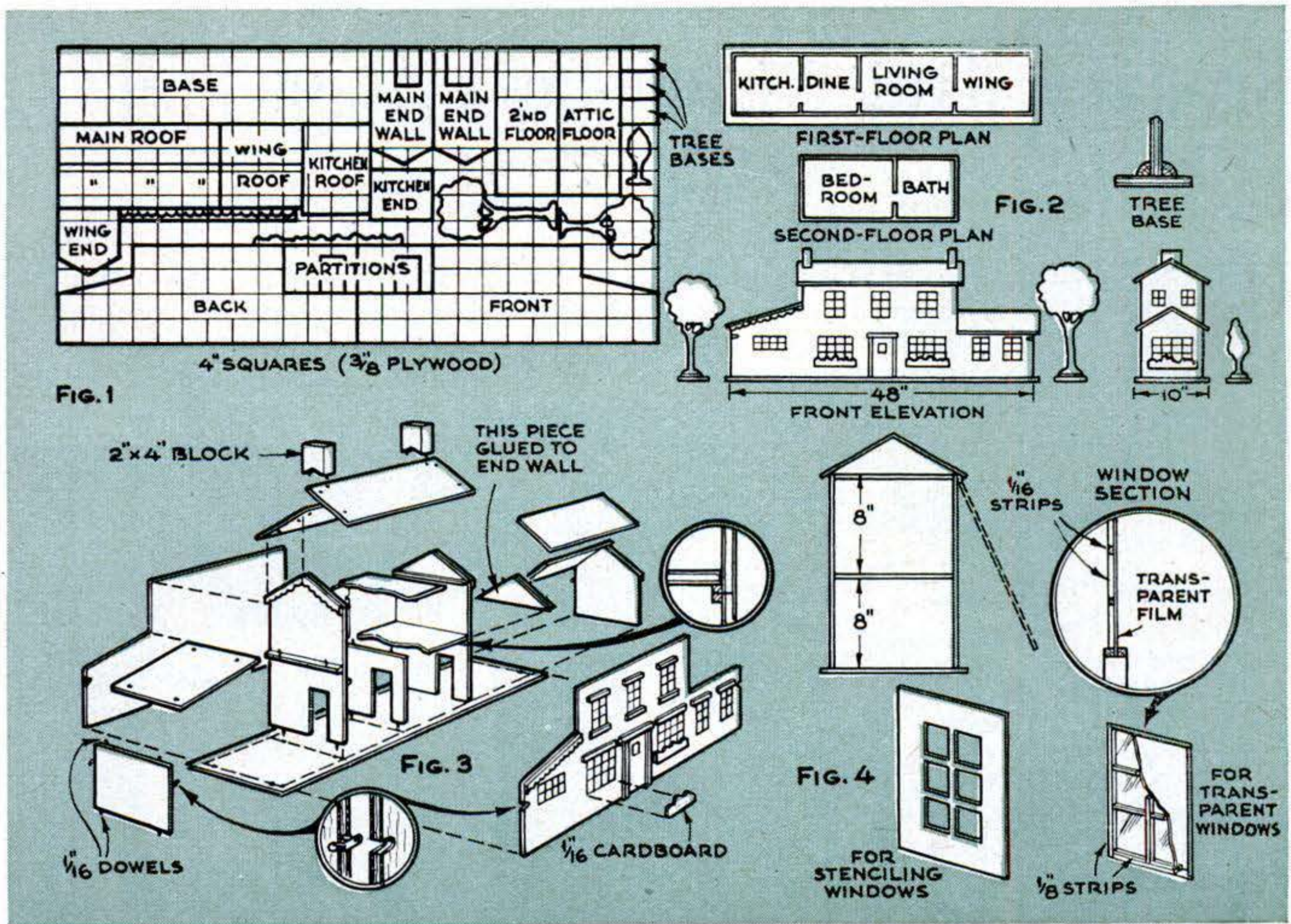
All structural parts of this doll house are cut from a single 4' by 8' sheet of \frac{3}{8} " plywood.
